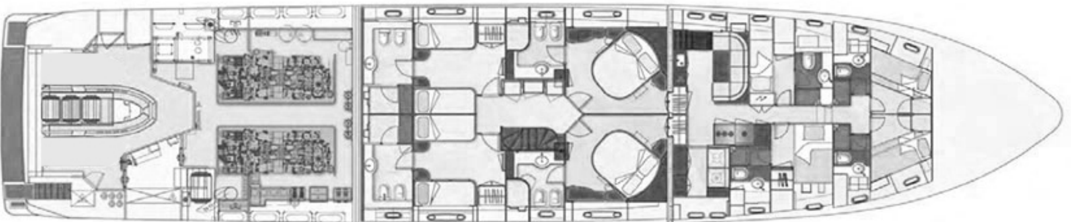
LOWER DECK
